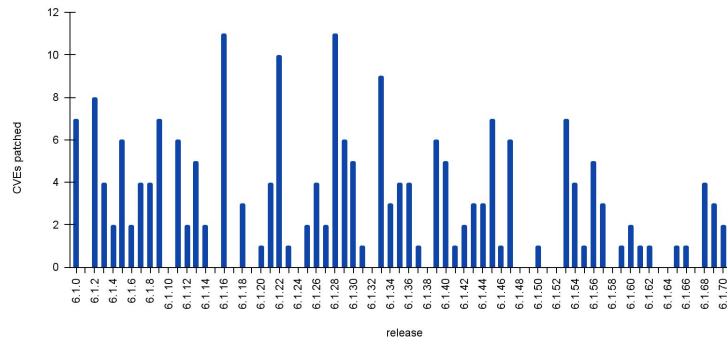
CVEs fixed per release for 6.1.x branch
