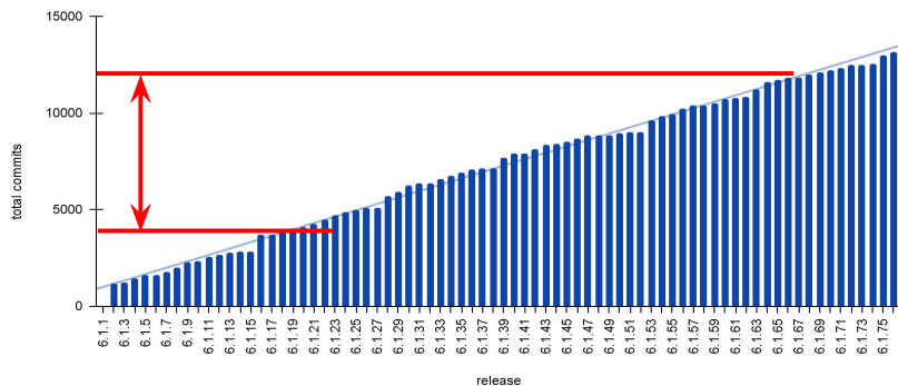
Total commits per release for 6.1.x branch
